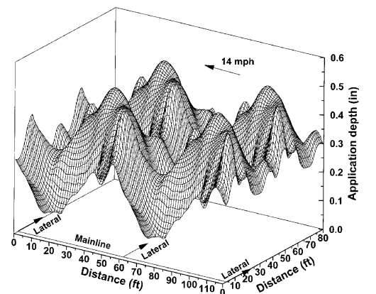
Figure 9. Combined application pattern from nine sprinklers with a 40 ft sprinkler spacing and 60 ft lateral spacing in a 14 mph wind oriented perpendicular to the laterals.
